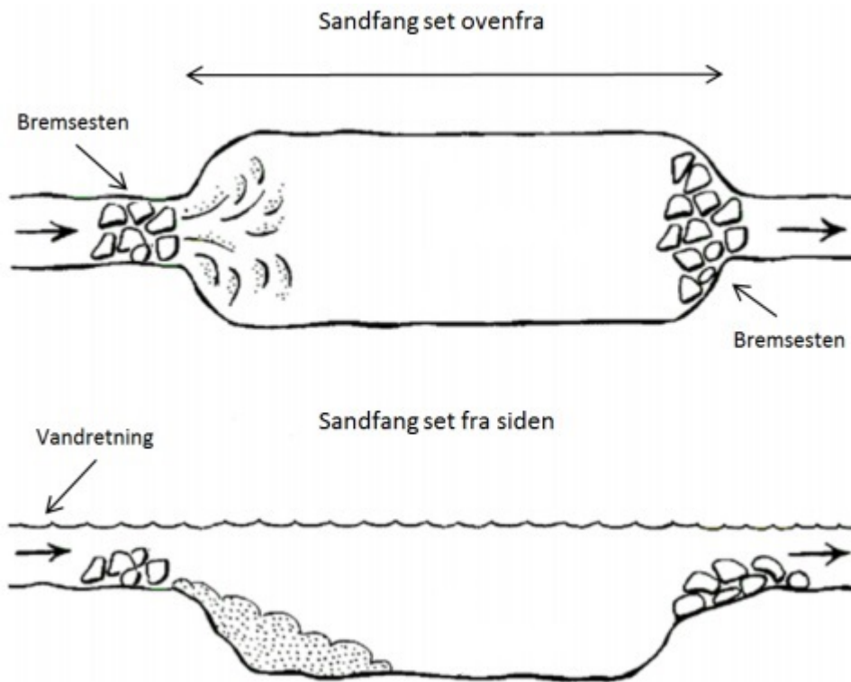
Figur 1: Principskitse for etablering af sandfang
