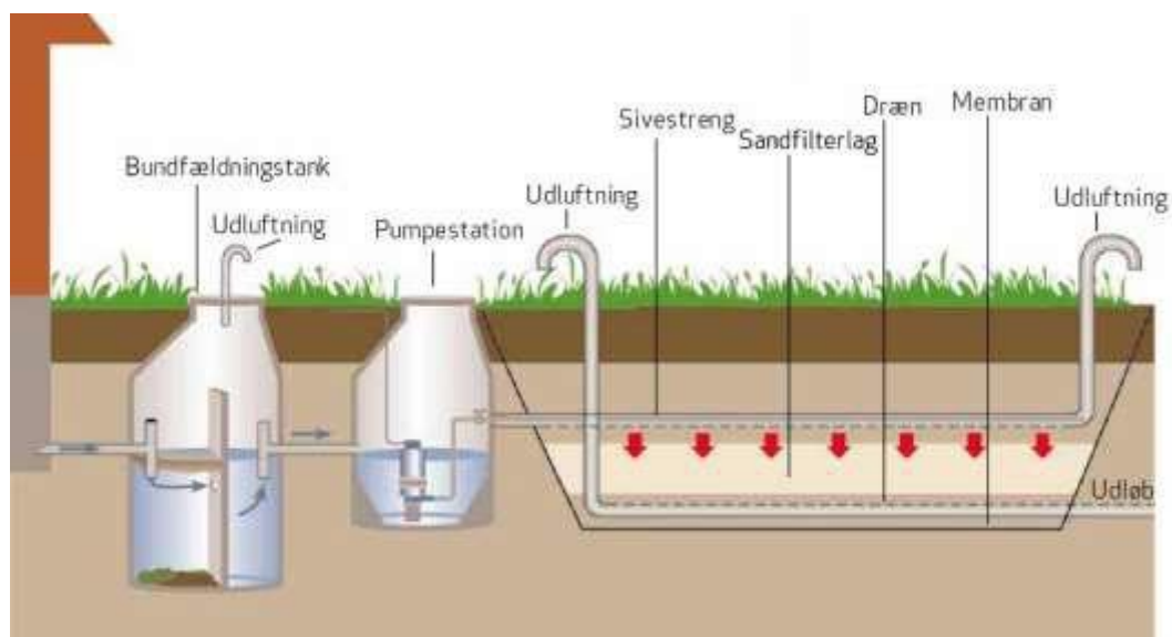
Figur 5. Biologisk sandfilter.
